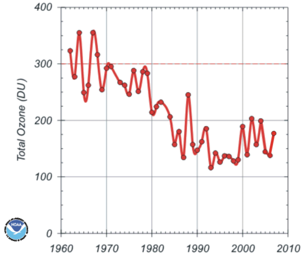
South Pole Dobson Ozone Spectrophotometer October 15-31 Average
